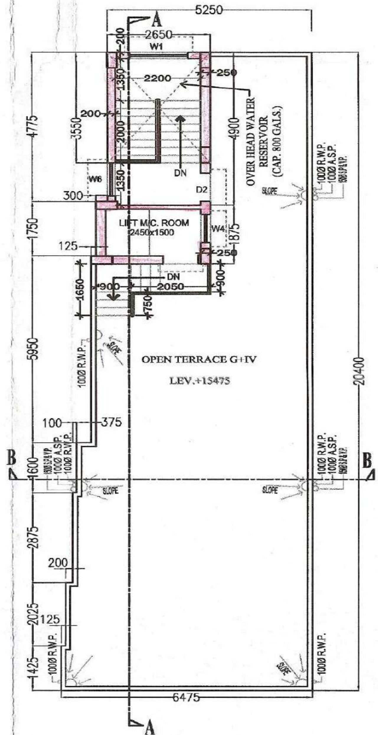
ROOF R PLAN
